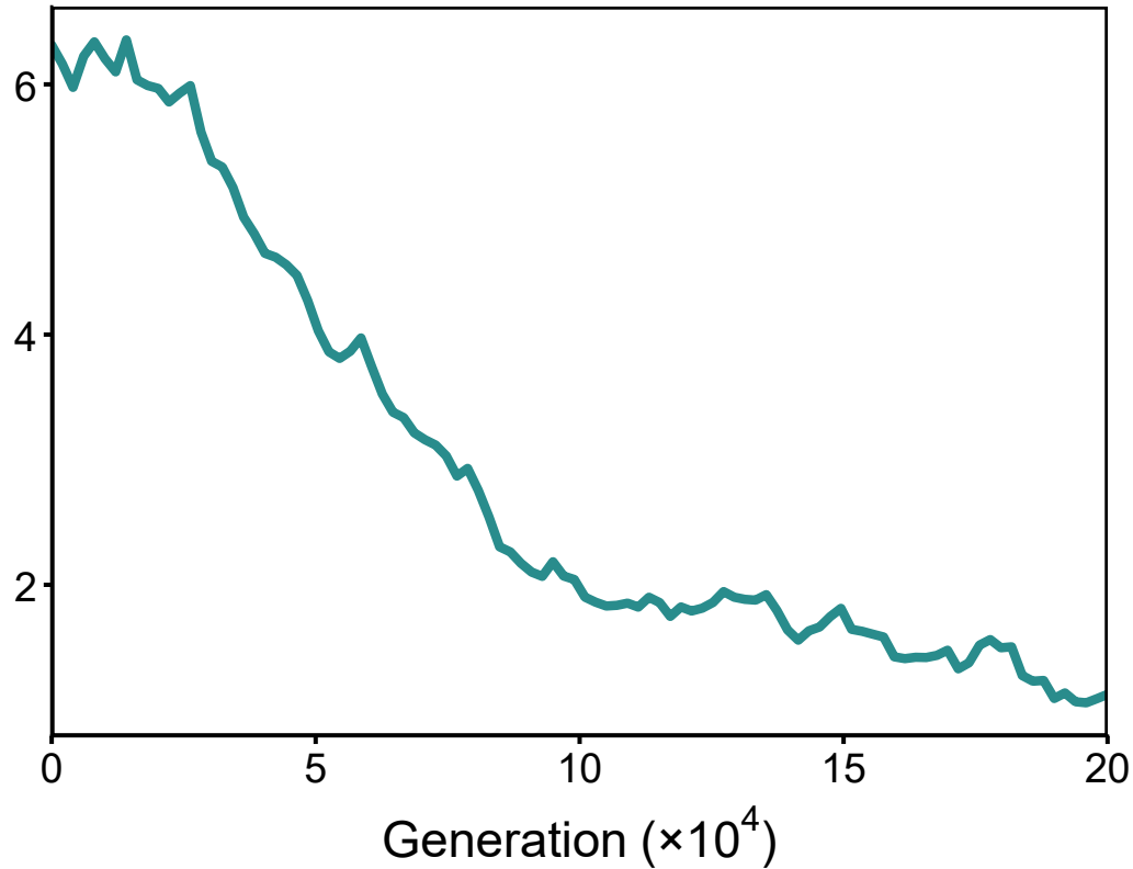
Mean absolute deviation from the true coefficient
